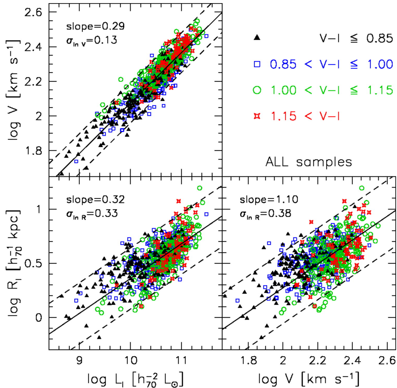
Fig. 5. from Scaling Relations of Spiral Galaxies Courteau et al. 2007 ApJ 671 203 doi:10.1086/522193 https://dx.doi.org/10.1086/522193
