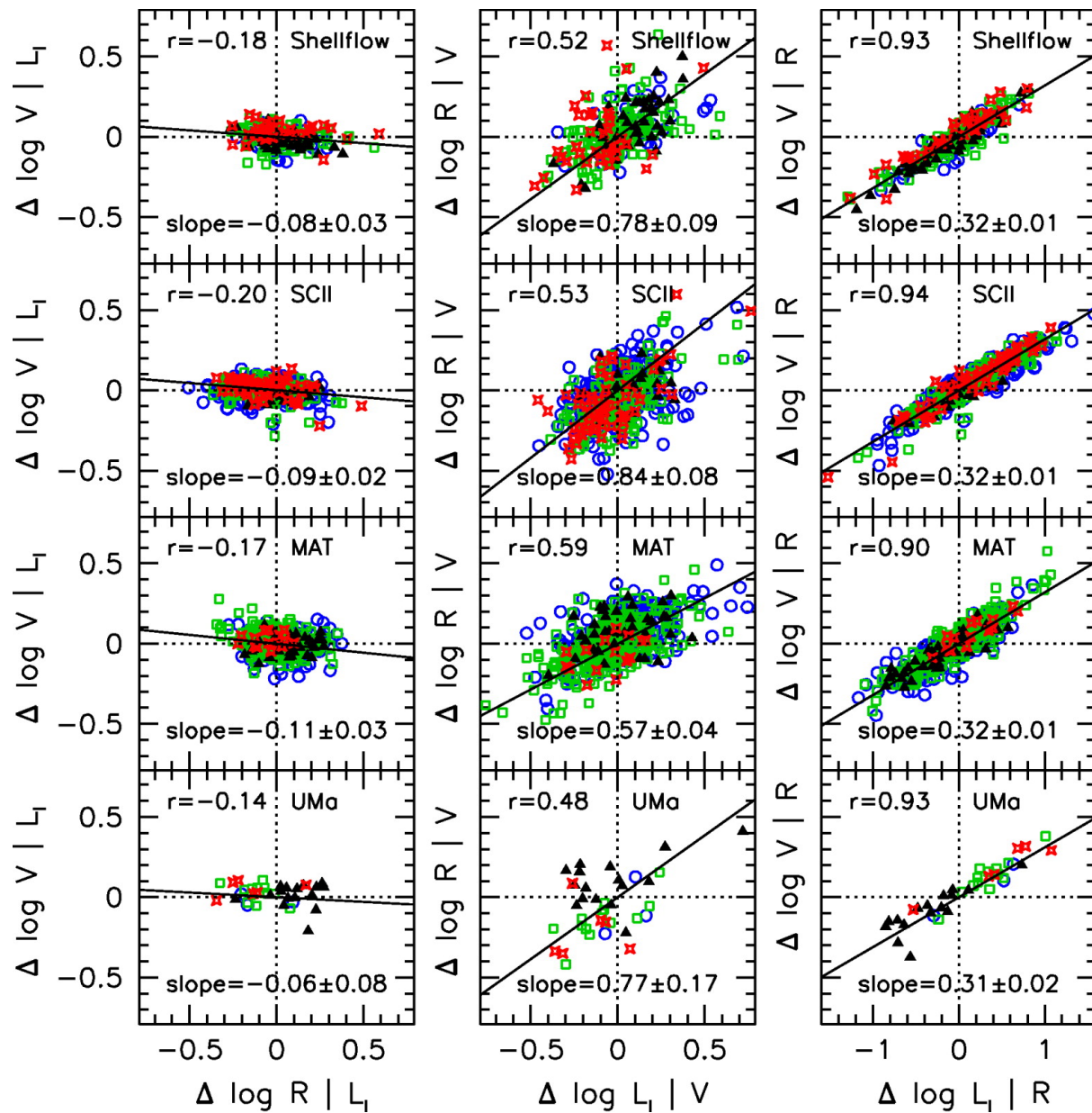
Fig. 18. from Scaling Relations of Spiral Galaxies Courteau et al. 2007 ApJ 671 203 doi:10.1086/522193 https://dx.doi.org/10.1086/522193
