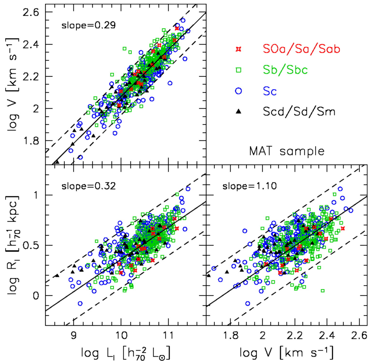
Fig. 15. from Scaling Relations of Spiral Galaxies Courteau et al. 2007 ApJ 671 203 doi:10.1086/522193 https://dx.doi.org/10.1086/522193
