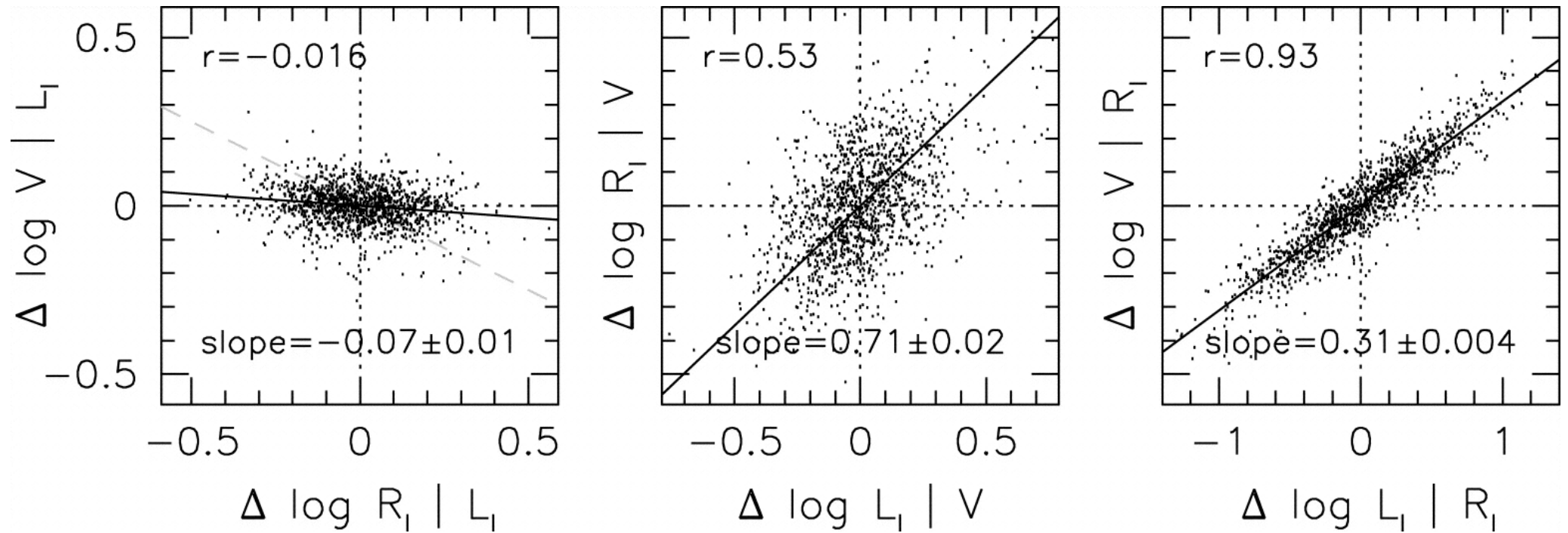
Fig. 12. from Scaling Relations of Spiral Galaxies Courteau et al. 2007 ApJ 671 203 doi:10.1086/522193 https://dx.doi.org/10.1086/522193
