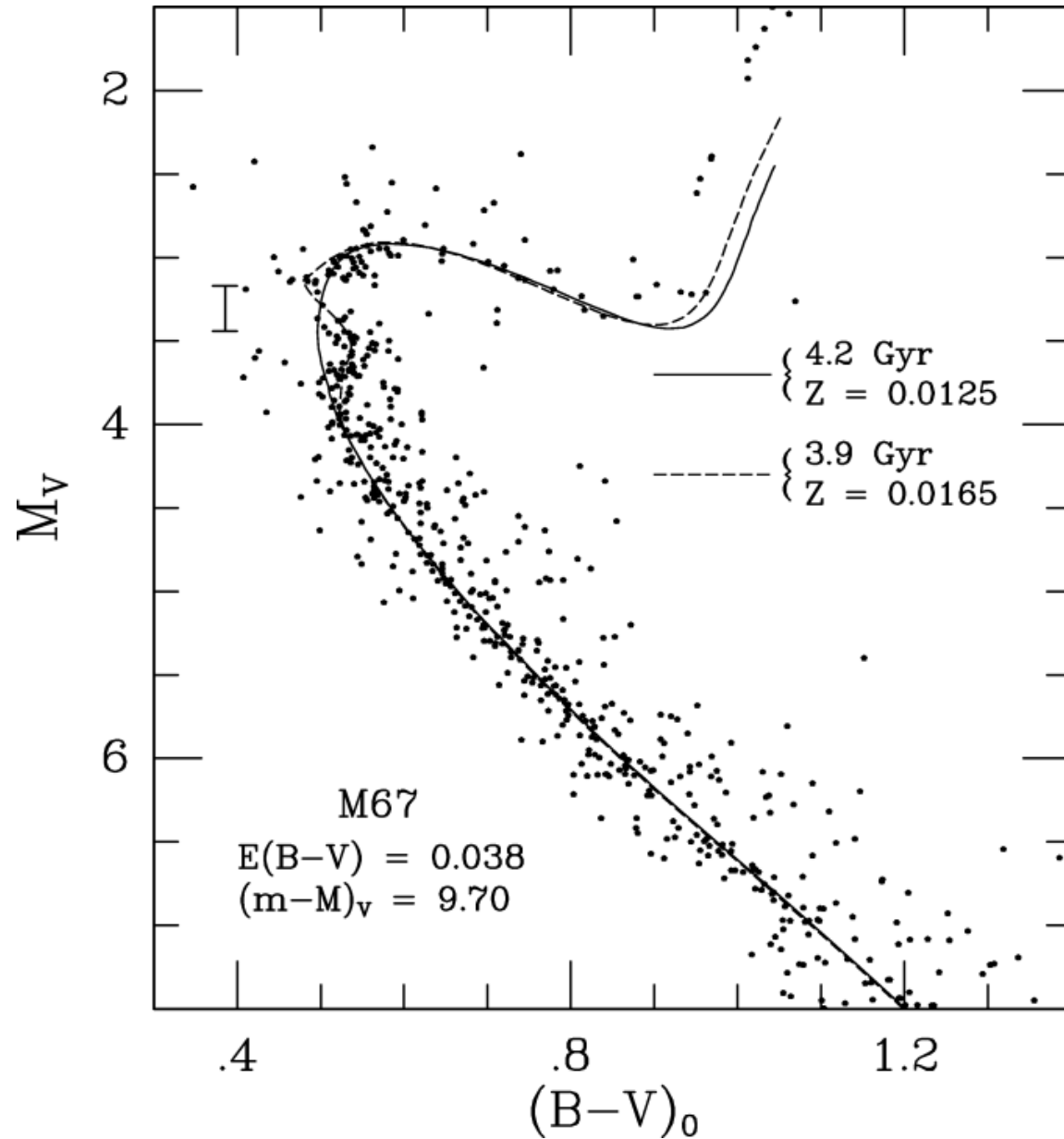
Fig. 2. from A Constraint on Z from Fits of Isochrones to the ColorMagnitude Diagram of M67 VandenBerg et al. 2007 ApJL 666 L105 doi:10.1086/521877 https://dx.doi.org/10.1086/521877
