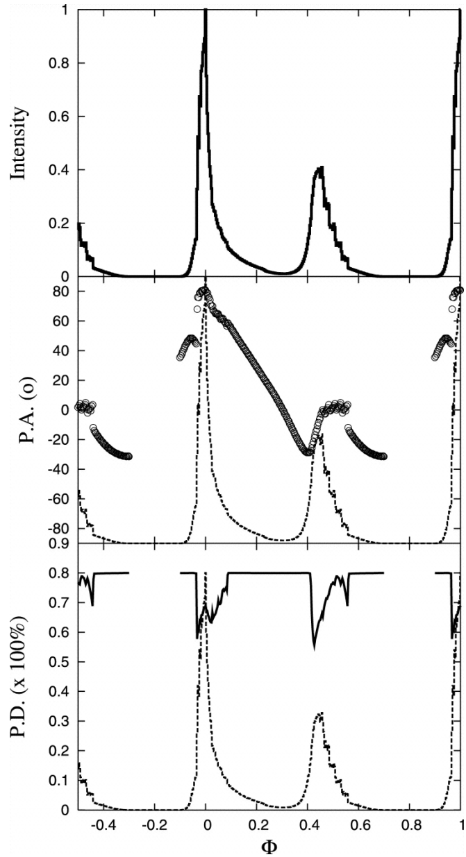
Fig. 9. from Pulse Profiles, Spectra, and Polarization Characteristics of Nonthermal Emissions from the Crablike Pulsars Takata & Chang 2007 ApJ 670 677 doi:10.1086/521785 https://dx.doi.org/10.1086/521785
