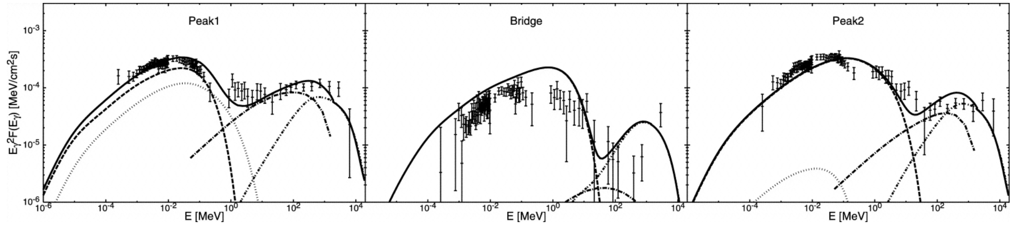
Fig. 6. from Pulse Profiles, Spectra, and Polarization Characteristics of Nonthermal Emissions from the Crablike Pulsars Takata & Chang 2007 ApJ 670 677 doi:10.1086/521785 https://dx.doi.org/10.1086/521785 © 2007. The American Astronomical Society. All rights reserved. Printed in U.S.A.
