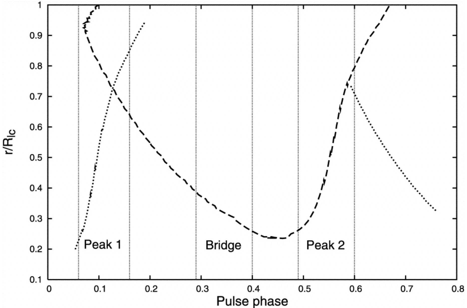
Fig. 5. from Pulse Profiles, Spectra, and Polarization Characteristics of Nonthermal Emissions from the Crablike Pulsars Takata & Chang 2007 ApJ 670 677 doi:10.1086/521785 https://dx.doi.org/10.1086/521785 © 2007. The American Astronomical Society. All rights reserved. Printed in U.S.A.
