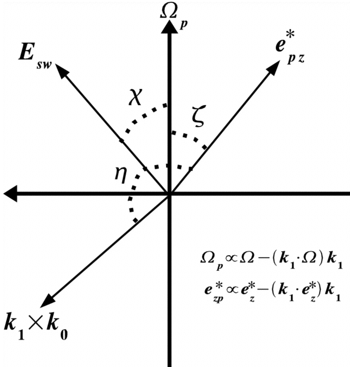
Fig. 3. from Pulse Profiles, Spectra, and Polarization Characteristics of Nonthermal Emissions from the Crablike Pulsars Takata & Chang 2007 ApJ 670 677 doi:10.1086/521785 https://dx.doi.org/10.1086/521785 © 2007. The American Astronomical Society. All rights reserved. Printed in U.S.A.
