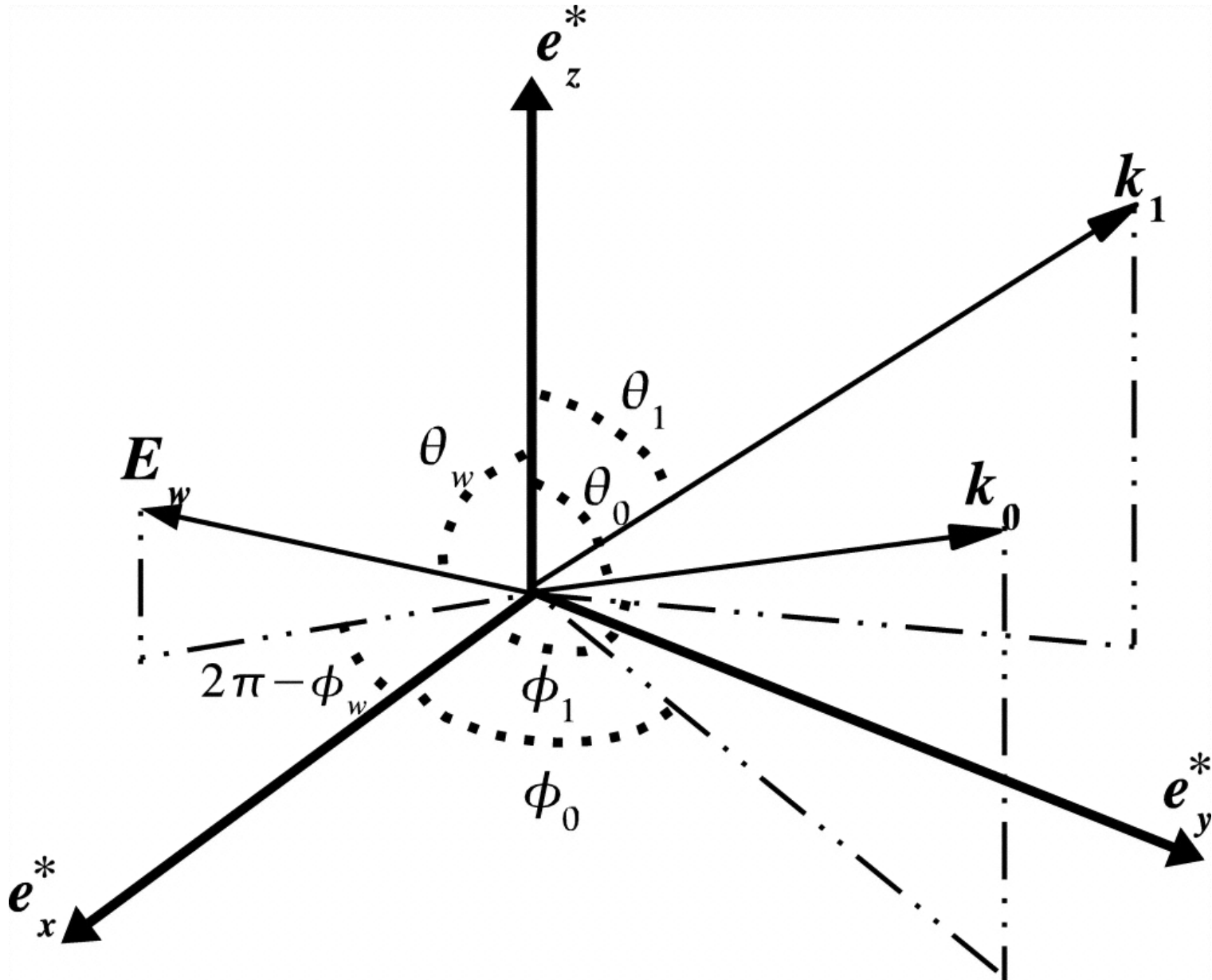
Fig. 3. from Pulse Profiles, Spectra, and Polarization Characteristics of Nonthermal Emissions from the Crablike Pulsars Takata & Chang 2007 ApJ 670 677 doi:10.1086/521785 https://dx.doi.org/10.1086/521785 © 2007. The American Astronomical Society. All rights reserved. Printed in U.S.A.
