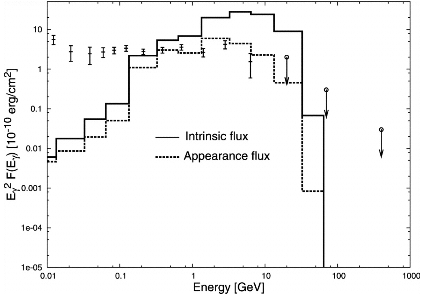
Fig. 2. from Pulse Profiles, Spectra, and Polarization Characteristics of Nonthermal Emissions from the Crablike Pulsars Takata & Chang 2007 ApJ 670 677 doi:10.1086/521785 https://dx.doi.org/10.1086/521785 © 2007. The American Astronomical Society. All rights reserved. Printed in U.S.A.
