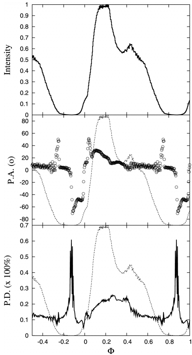
Fig. 11. from Pulse Profiles, Spectra, and Polarization Characteristics of Nonthermal Emissions from the Crablike Pulsars Takata & Chang 2007 ApJ 670 677 doi:10.1086/521785 https://dx.doi.org/10.1086/521785
