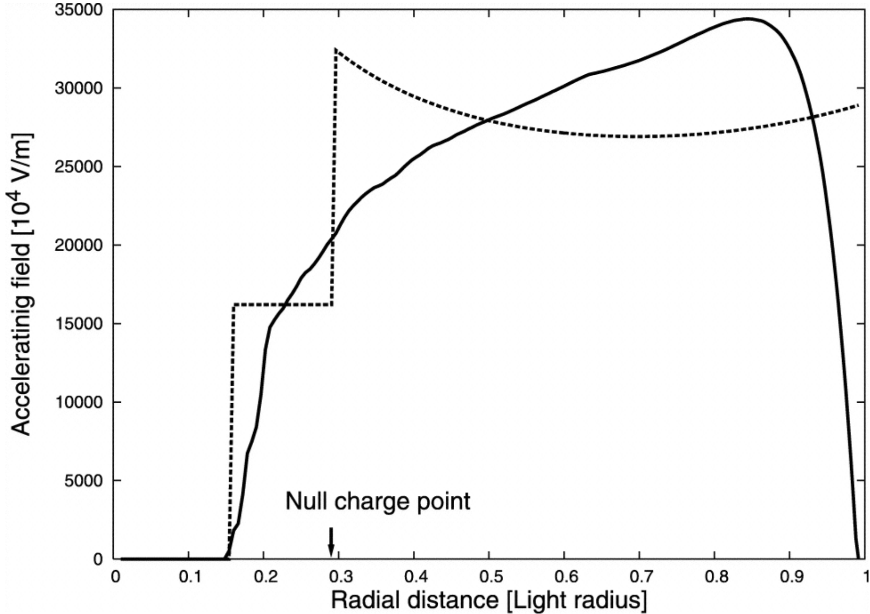
Fig. 1. from Pulse Profiles, Spectra, and Polarization Characteristics of Nonthermal Emissions from the Crablike Pulsars Takata & Chang 2007 ApJ 670 677 doi:10.1086/521785 https://dx.doi.org/10.1086/521785
