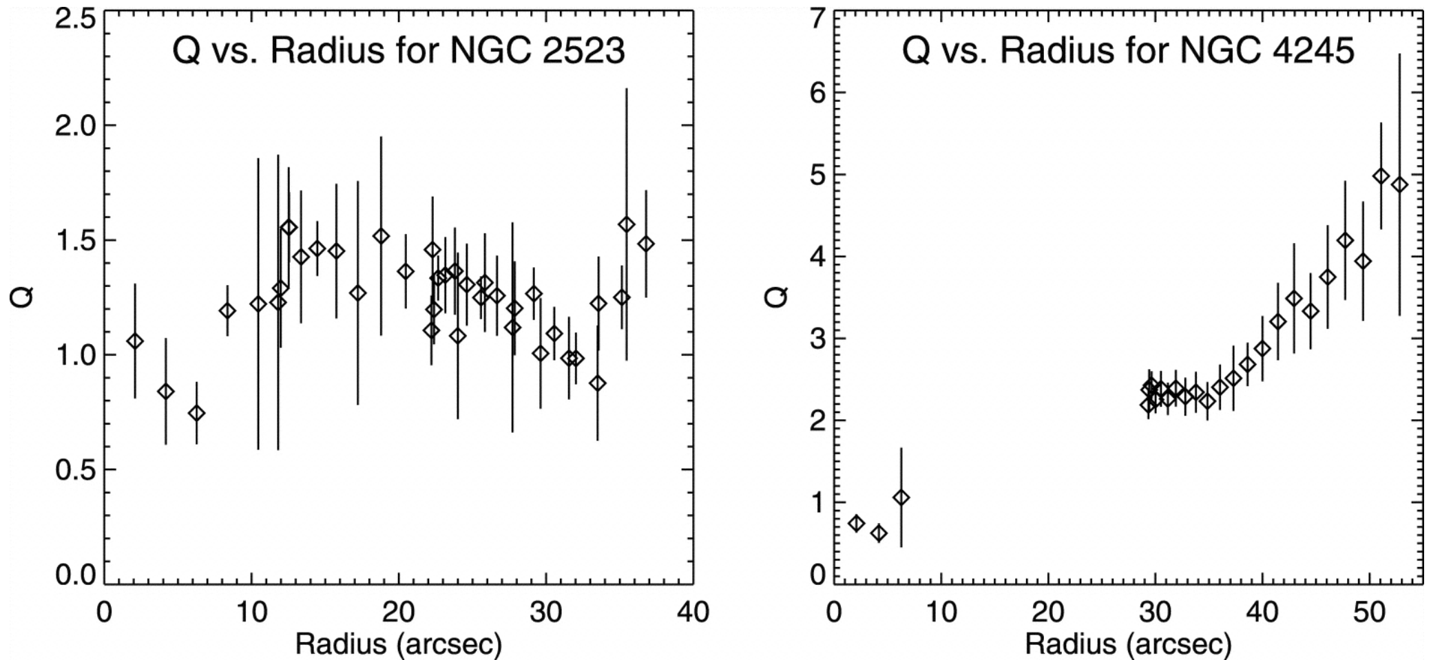
Fig. 9. from The Kinematically Measured Pattern Speeds of NGC 2523 and NGC 4245 Treuthardt et al. 2007 AJ 134 1195 doi:10.1086/521149 https://dx.doi.org/10.1086/521149 © 2007. The American Astronomical Society. All rights reserved. Printed in U.S.A.
