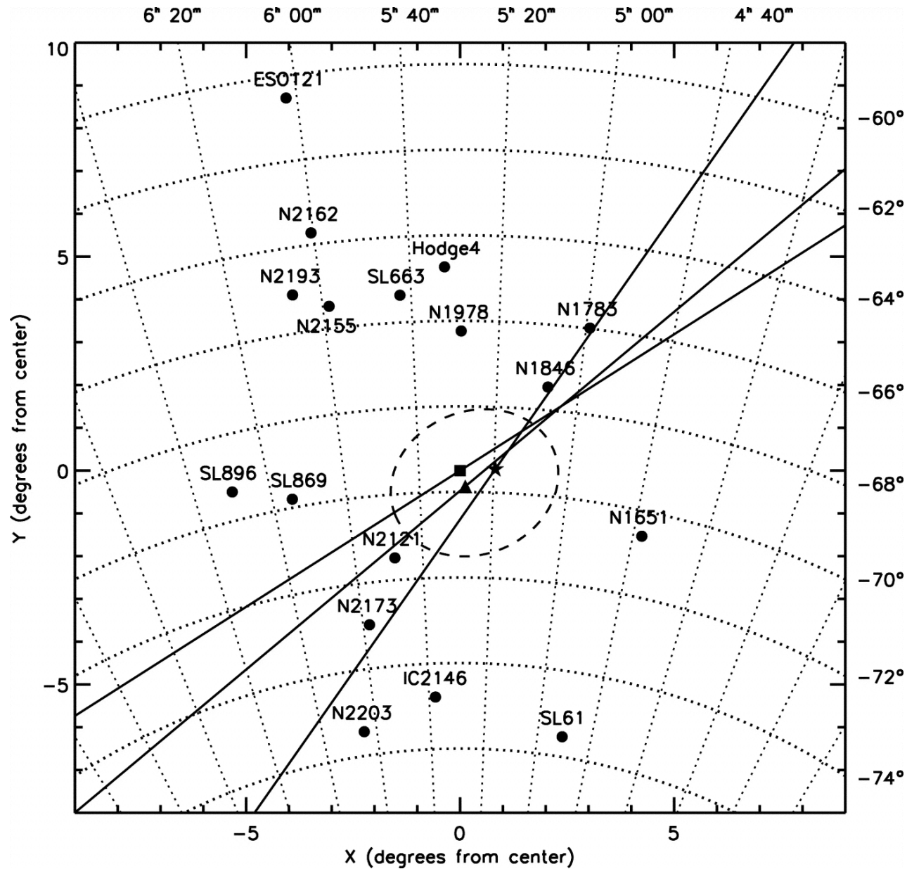
Fig. 4. from Distances to Populous Clusters in the Large Magellanic Cloud via the Kband Luminosity of the Red Clump Grocholski et al. 2007 AJ 134 680 doi:10.1086/519735 https://dx.doi.org/10.1086/519735
