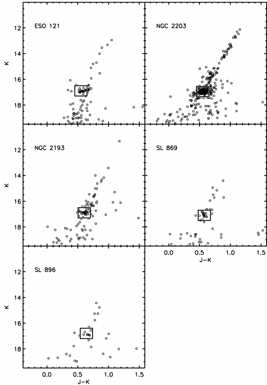
Fig. 3. from Distances to Populous Clusters in the Large Magellanic Cloud via the Kband Luminosity of the Red Clump Grocholski et al. 2007 AJ 134 680 doi:10.1086/519735 https://dx.doi.org/10.1086/519735
