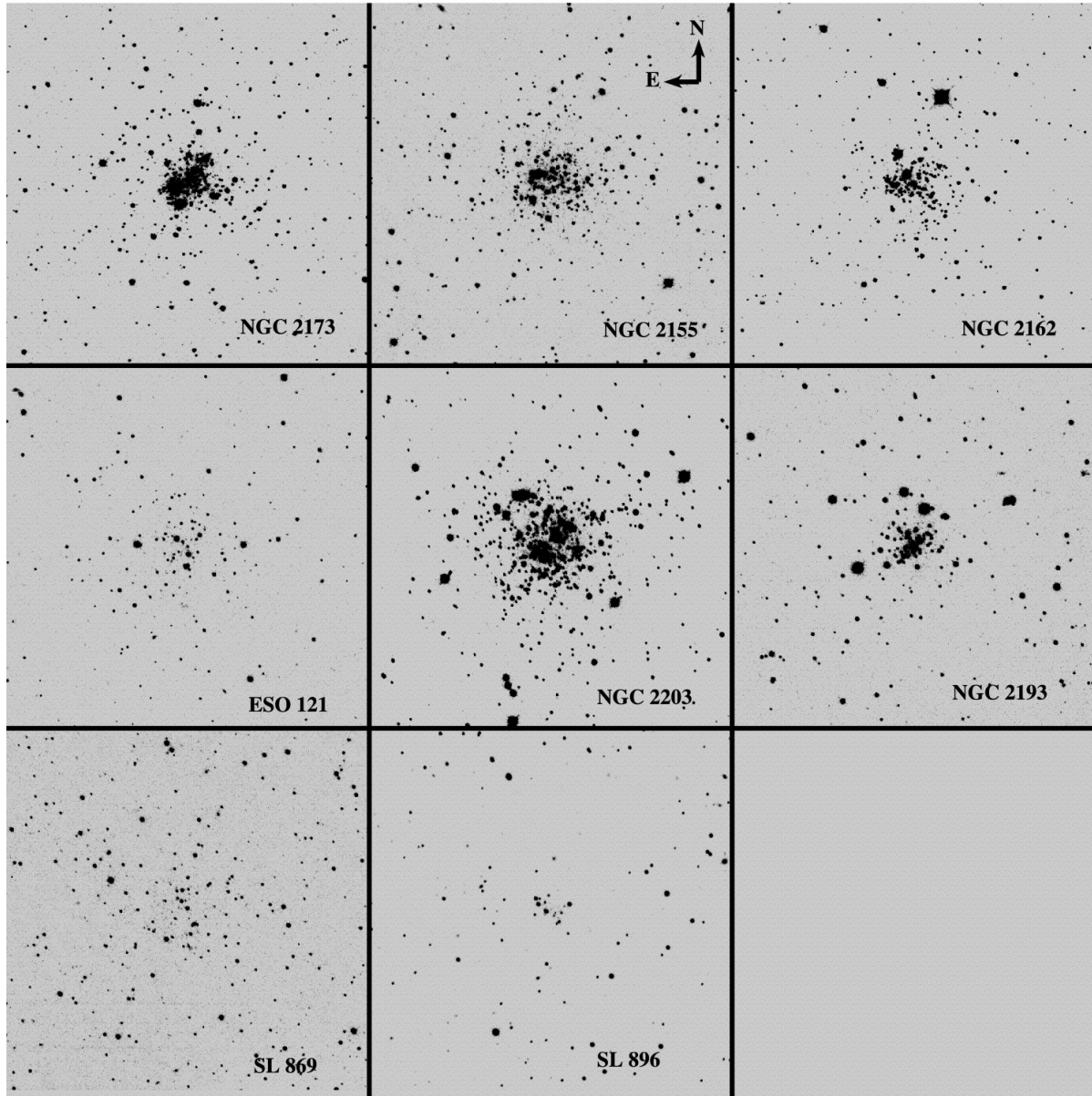
Fig. 1. from Distances to Populous Clusters in the Large Magellanic Cloud via the Kband Luminosity of the Red Clump Grocholski et al. 2007 AJ 134 680 doi:10.1086/519735 https://dx.doi.org/10.1086/519735 © 2007. The American Astronomical Society. All rights reserved. Printed in U.S.A.
