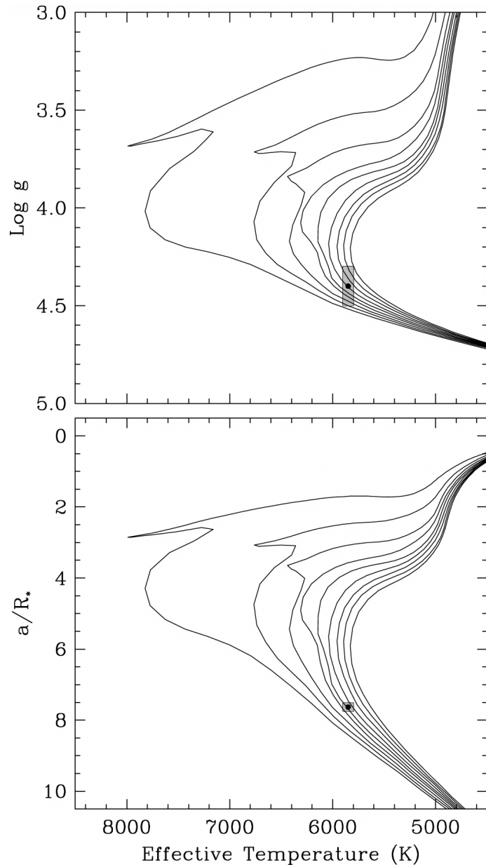
Fig. 4. from Improving Stellar and Planetary Parameters of Transiting Planet Systems: The Case of TrES2 Sozzetti et al. 2007 ApJ 664 1190 doi:10.1086/519214 https://dx.doi.org/10.1086/519214
