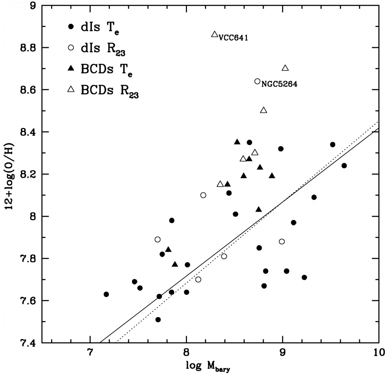
Fig. 9. from Chemical Properties of StarForming Dwarf Galaxies Vaduvescu, McCall, & Richer 2007 AJ 134 604 doi:10.1086/518865 https://dx.doi.org/10.1086/518865
