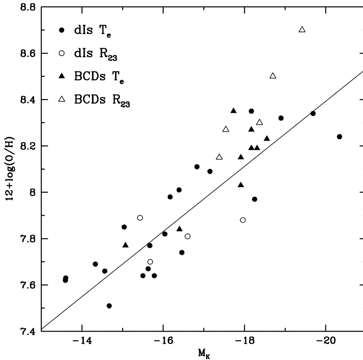
Fig. 7. from Chemical Properties of StarForming Dwarf Galaxies Vaduvescu, McCall, & Richer 2007 AJ 134 604 doi:10.1086/518865 https://dx.doi.org/10.1086/518865
