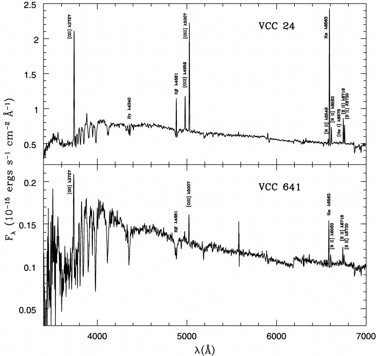
Fig. 3. from Chemical Properties of StarForming Dwarf Galaxies Vaduvescu, McCall, & Richer 2007 AJ 134 604 doi:10.1086/518865 https://dx.doi.org/10.1086/518865
