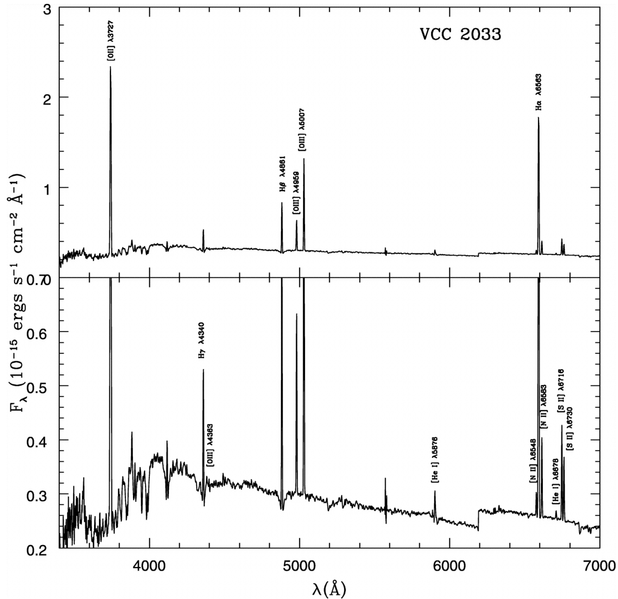
Fig. 2. from Chemical Properties of StarForming Dwarf Galaxies Vaduvescu, McCall, & Richer 2007 AJ 134 604 doi:10.1086/518865 https://dx.doi.org/10.1086/518865
