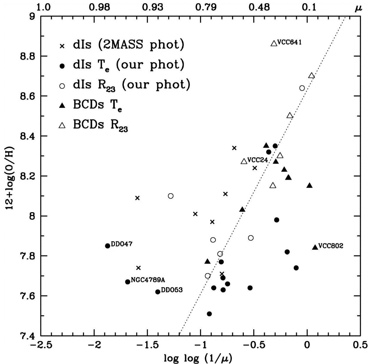
Fig. 10. from Chemical Properties of StarForming Dwarf Galaxies Vaduvescu, McCall, & Richer 2007 AJ 134 604 doi:10.1086/518865 https://dx.doi.org/10.1086/518865
