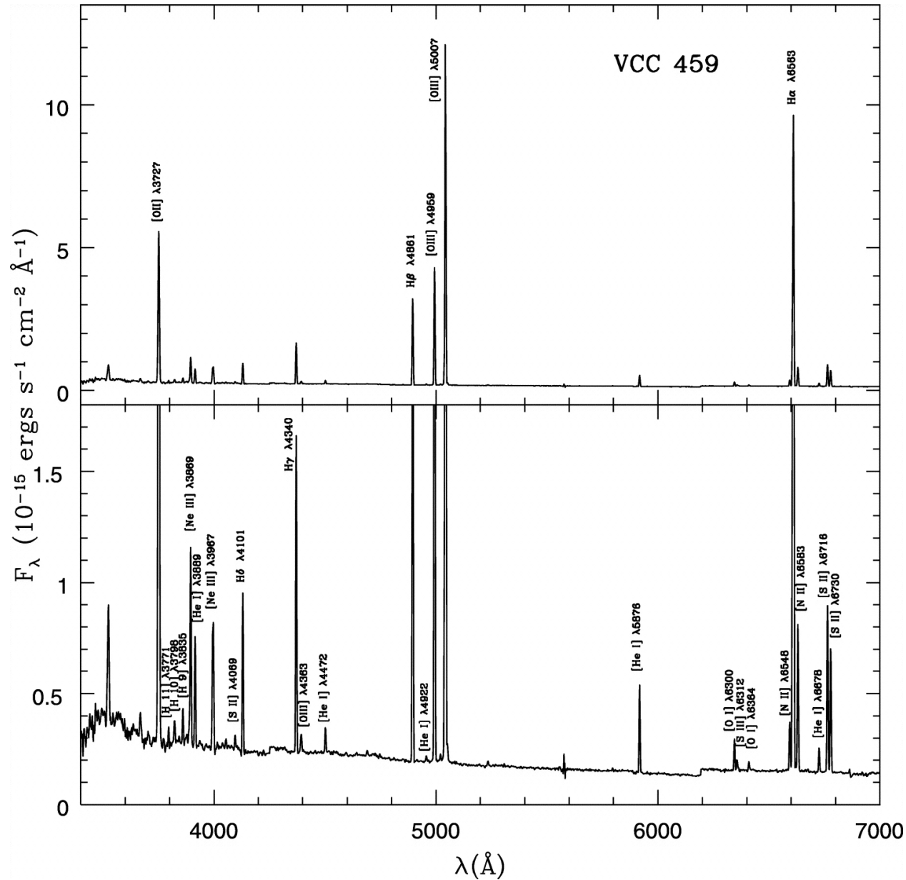
Fig. 1. from Chemical Properties of StarForming Dwarf Galaxies Vaduvescu, McCall, & Richer 2007 AJ 134 604 doi:10.1086/518865 https://dx.doi.org/10.1086/518865
