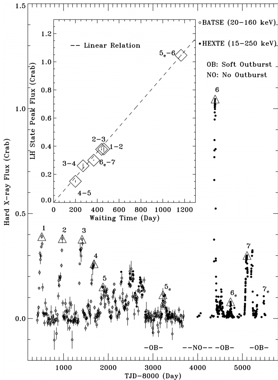
Fig. 3. from Peak Luminosities of the Hard States of GX 3394: Implications for the Accretion Geometry, Disk Mass, and Black Hole Mass Yu et al. 2007 ApJ 663 1309 doi:10.1086/518733 https://dx.doi.org/10.1086/518733 © 2007. The American Astronomical Society. All rights reserved. Printed in U.S.A.
