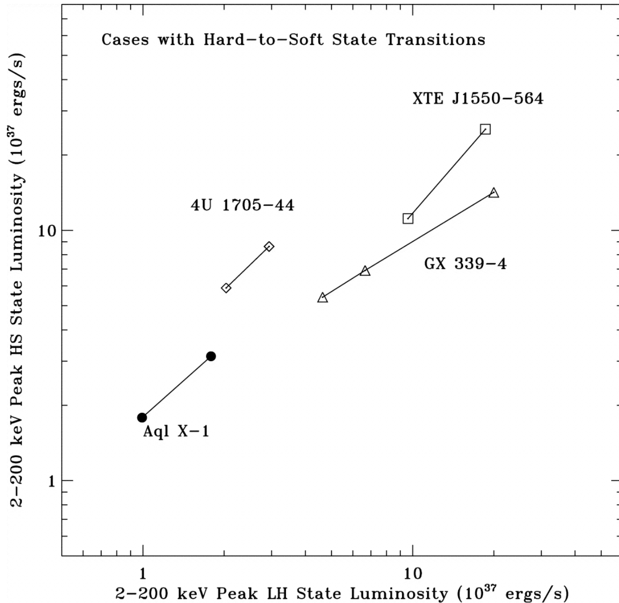
Fig. 2. from Peak Luminosities of the Hard States of GX 3394: Implications for the Accretion Geometry, Disk Mass, and Black Hole Mass Yu et al. 2007 ApJ 663 1309 doi:10.1086/518733 https://dx.doi.org/10.1086/518733 © 2007. The American Astronomical Society. All rights reserved. Printed in U.S.A.
