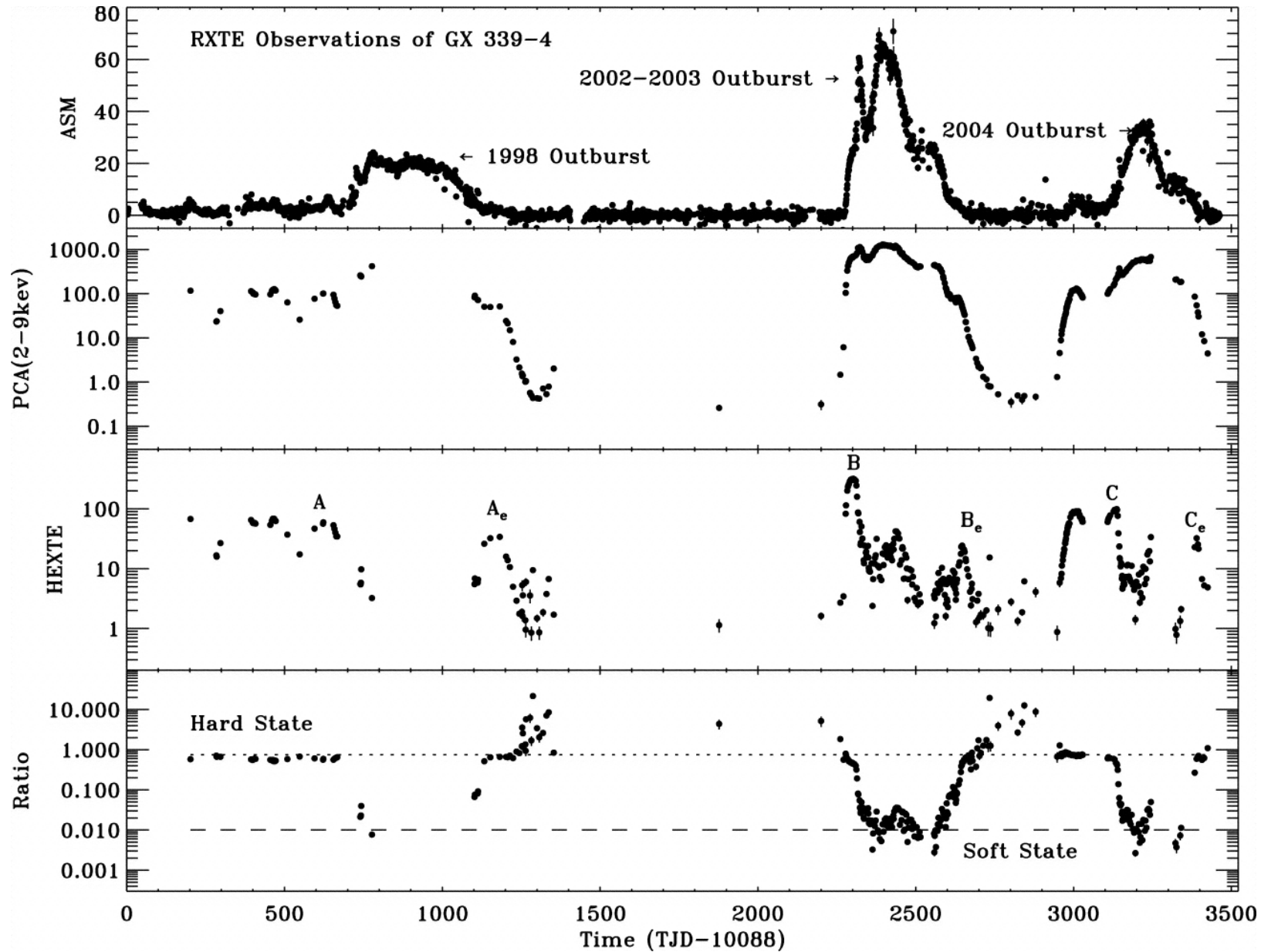
Fig. 1. from Peak Luminosities of the Hard States of GX 3394: Implications for the Accretion Geometry, Disk Mass, and Black Hole Mass Yu et al. 2007 ApJ 663 1309 doi:10.1086/518733 https://dx.doi.org/10.1086/518733
