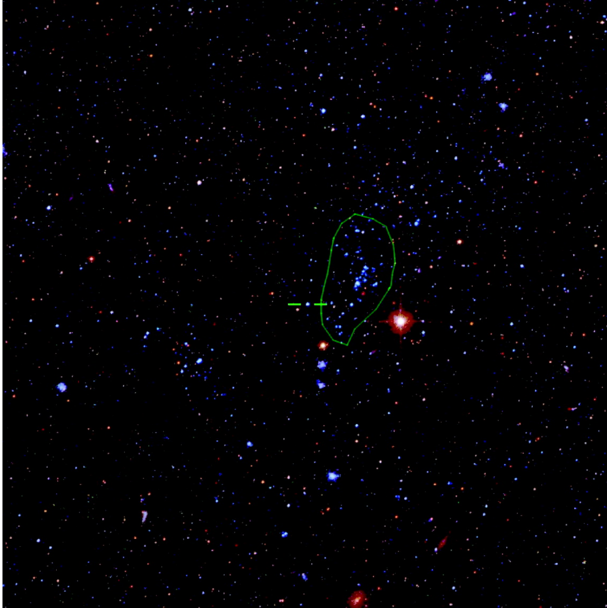
Fig. 5. from Optical Studies of the Ultraluminous XRay Source NGC 1313 X2 Liu et al. 2007 ApJ 661 165 doi:10.1086/516624 https://dx.doi.org/10.1086/516624 © 2007. The American Astronomical Society. All rights reserved. Printed in U.S.A.
