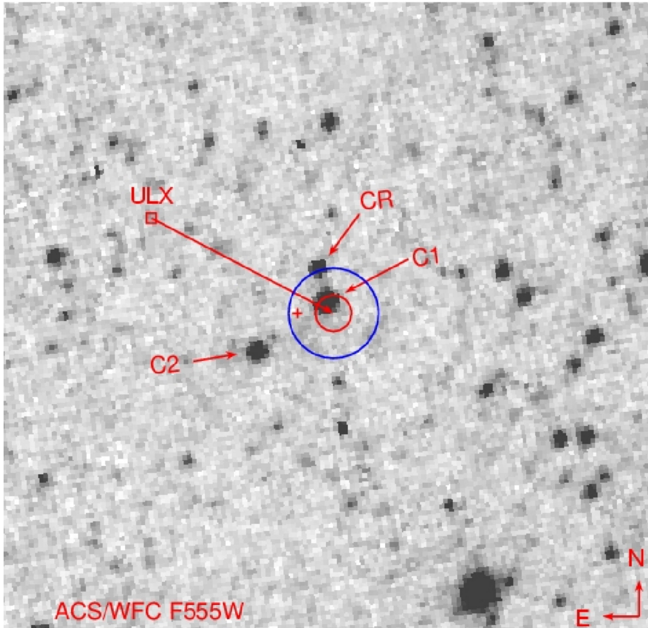
Fig. 1. from Optical Studies of the Ultraluminous XRay Source NGC 1313 X2 Liu et al. 2007 ApJ 661 165 doi:10.1086/516624 https://dx.doi.org/10.1086/516624 © 2007. The American Astronomical Society. All rights reserved. Printed in U.S.A.
