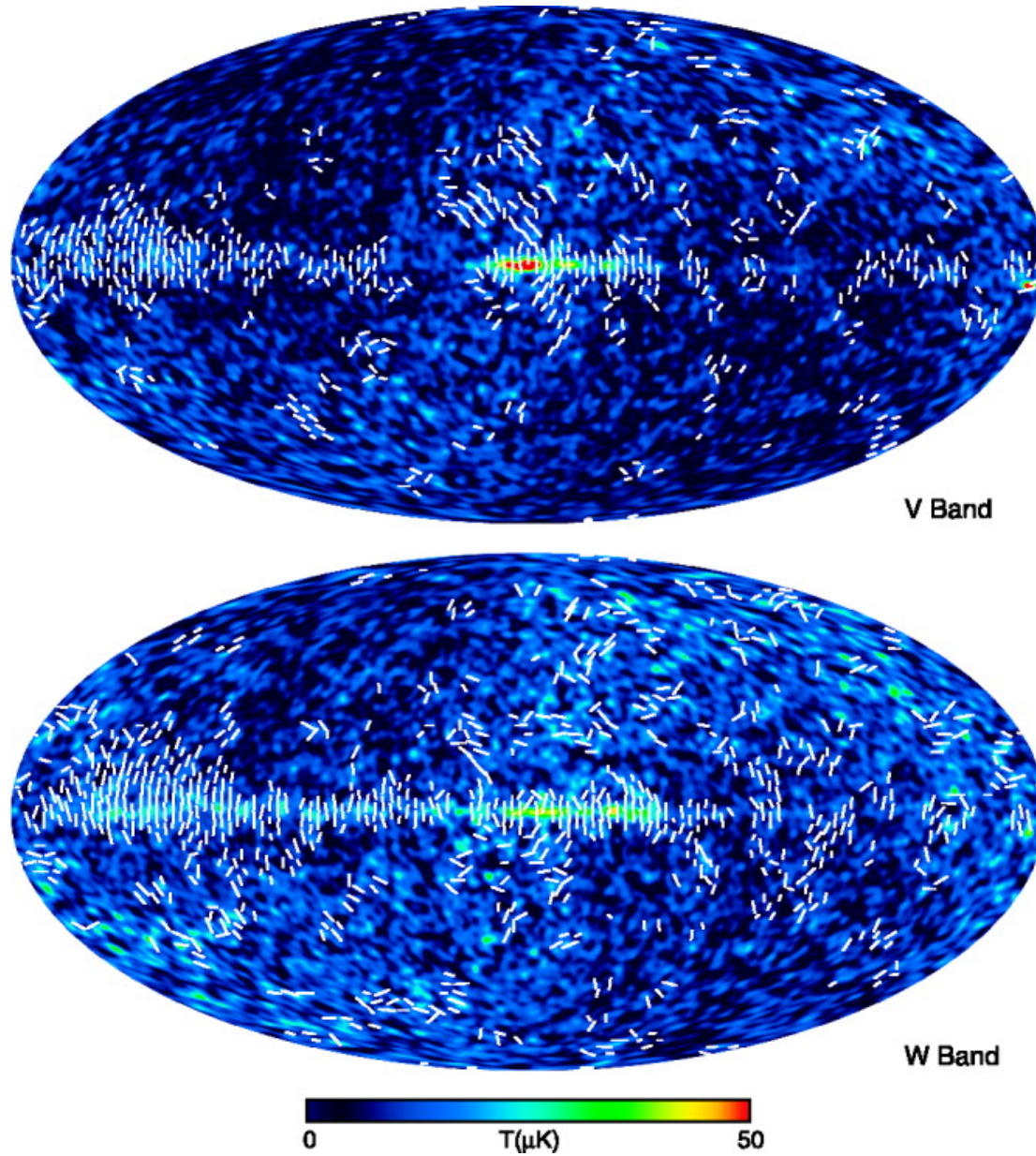
Fig. 4. from ThreeYear Wilkinson Microwave Anisotropy Probe (WMAP) Observations: Polarization Analysis Page et al. 2007 ApJS 170 335 doi:10.1086/513699 https://dx.doi.org/10.1086/513699 © 2007. The American Astronomical Society. All rights reserved. Printed in U.S.A.
