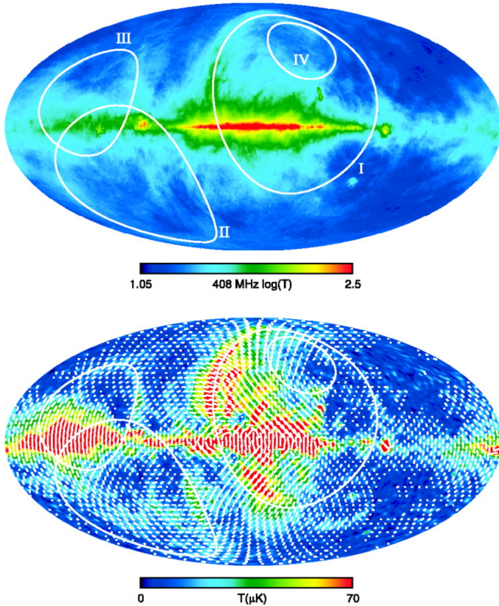
Fig. 10. from ThreeYear Wilkinson Microwave Anisotropy Probe (WMAP) Observations: Polarization Analysis Page et al. 2007 ApJS 170 335 doi:10.1086/513699 https://dx.doi.org/10.1086/513699 © 2007. The American Astronomical Society. All rights reserved. Printed in U.S.A.
