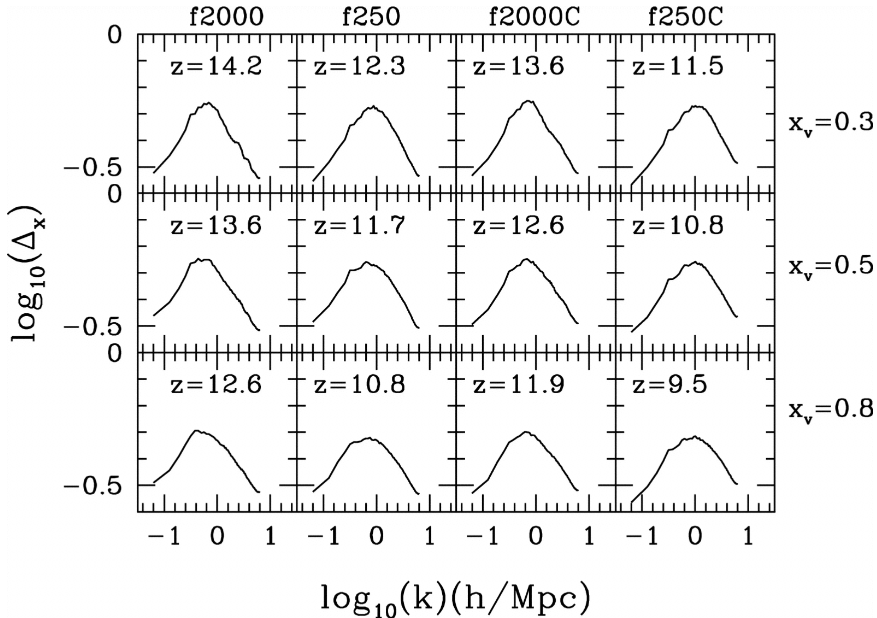
Fig. 9. from The Kinetic SunyaevZel'dovich Effect from Radiative Transfer Simulations of Patchy Reionization Iliev et al. 2007 ApJ 660 933 doi:10.1086/513687 https://dx.doi.org/10.1086/513687
