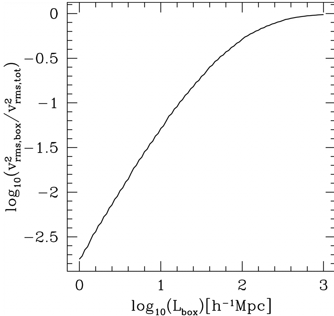
Fig. 7. from The Kinetic SunyaevZel'dovich Effect from Radiative Transfer Simulations of Patchy Reionization Iliev et al. 2007 ApJ 660 933 doi:10.1086/513687 https://dx.doi.org/10.1086/513687 © 2007. The American Astronomical Society. All rights reserved. Printed in U.S.A.
