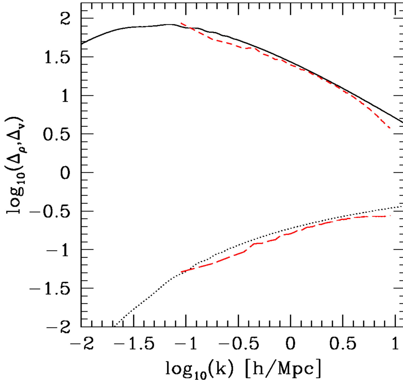
Fig. 6. from The Kinetic SunyaevZel'dovich Effect from Radiative Transfer Simulations of Patchy Reionization Iliev et al. 2007 ApJ 660 933 doi:10.1086/513687 https://dx.doi.org/10.1086/513687 © 2007. The American Astronomical Society. All rights reserved. Printed in U.S.A.
