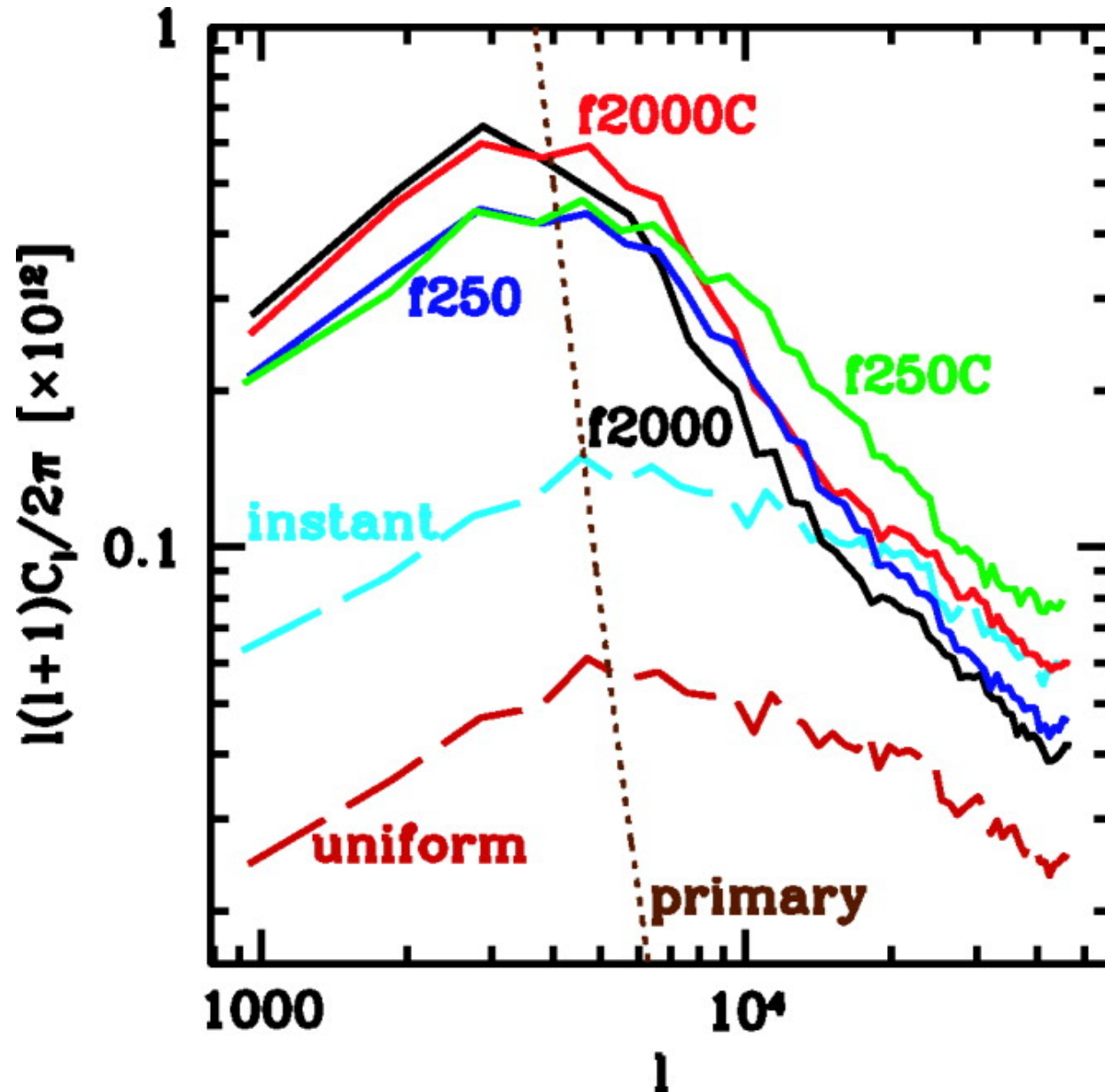
Fig. 4. from The Kinetic SunyaevZel'dovich Effect from Radiative Transfer Simulations of Patchy Reionization Iliev et al. 2007 ApJ 660 933 doi:10.1086/513687 https://dx.doi.org/10.1086/513687 © 2007. The American Astronomical Society. All rights reserved. Printed in U.S.A.
