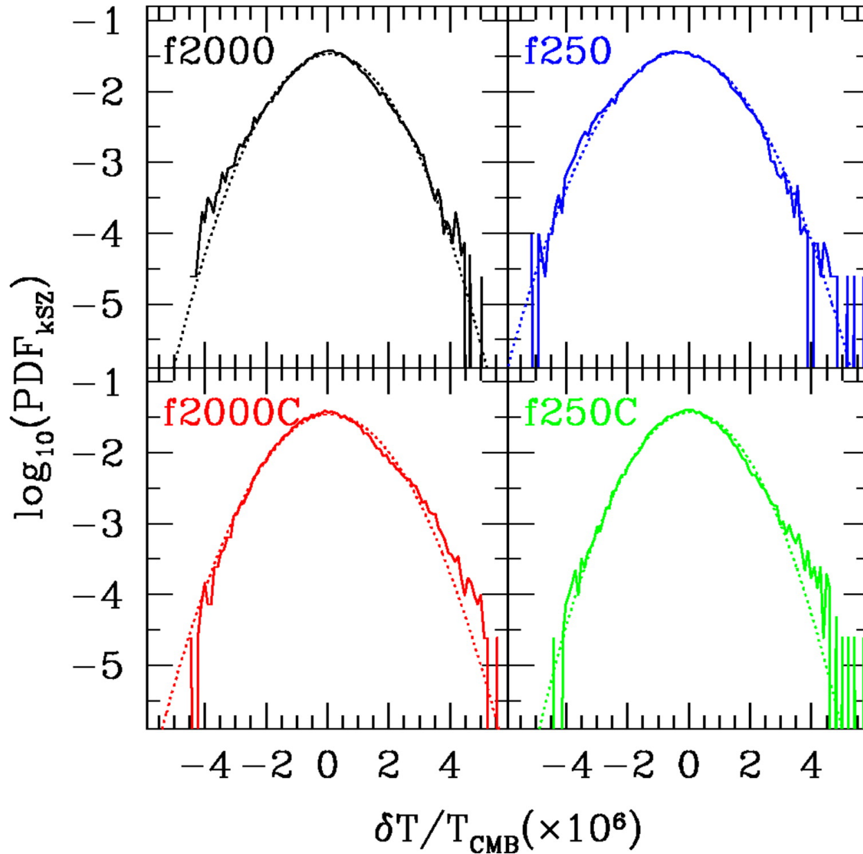
Fig. 2. from The Kinetic SunyaevZel'dovich Effect from Radiative Transfer Simulations of Patchy Reionization Iliev et al. 2007 ApJ 660 933 doi:10.1086/513687 https://dx.doi.org/10.1086/513687
