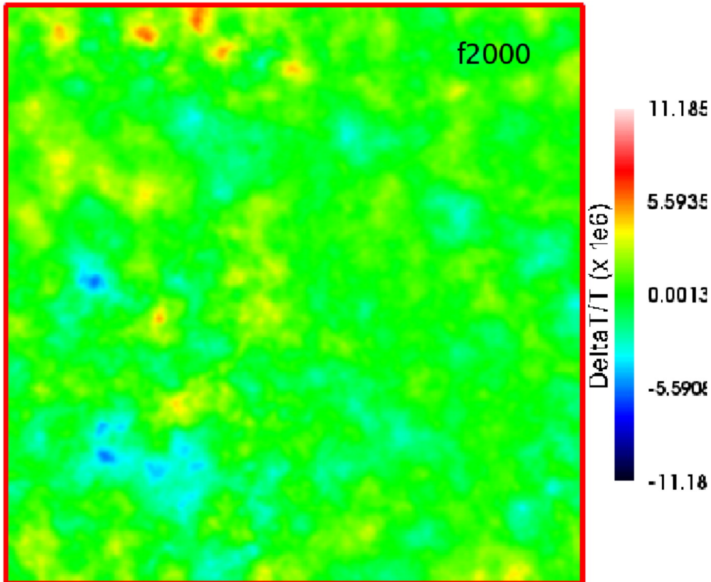
Fig. 1. from The Kinetic SunyaevZel'dovich Effect from Radiative Transfer Simulations of Patchy Reionization Iliev et al. 2007 ApJ 660 933 doi:10.1086/513687 https://dx.doi.org/10.1086/513687 © 2007. The American Astronomical Society. All rights reserved. Printed in U.S.A.
