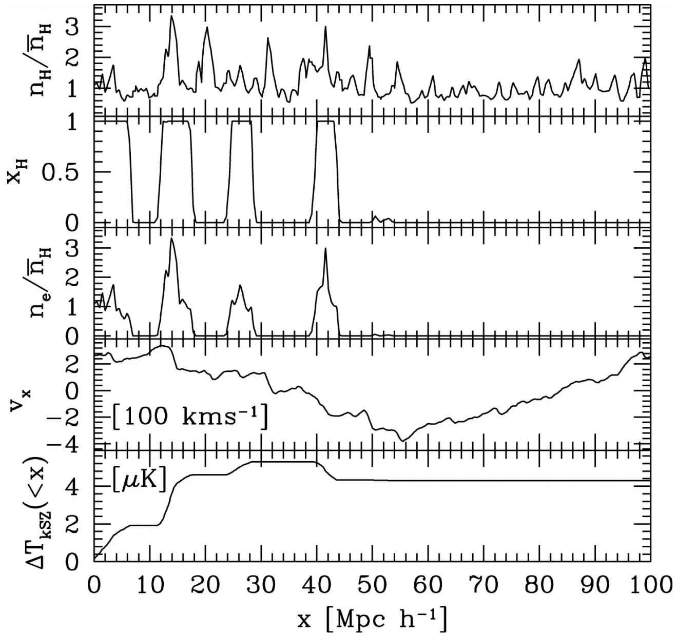
Fig. 12. from The Kinetic SunyaevZel'dovich Effect from Radiative Transfer Simulations of Patchy Reionization Iliev et al. 2007 ApJ 660 933 doi:10.1086/513687 https://dx.doi.org/10.1086/513687
