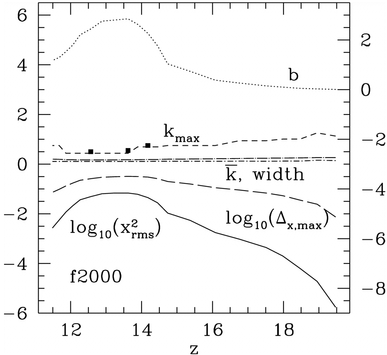
Fig. 10. from The Kinetic SunyaevZel'dovich Effect from Radiative Transfer Simulations of Patchy Reionization Iliev et al. 2007 ApJ 660 933 doi:10.1086/513687 https://dx.doi.org/10.1086/513687 © 2007. The American Astronomical Society. All rights reserved. Printed in U.S.A.
