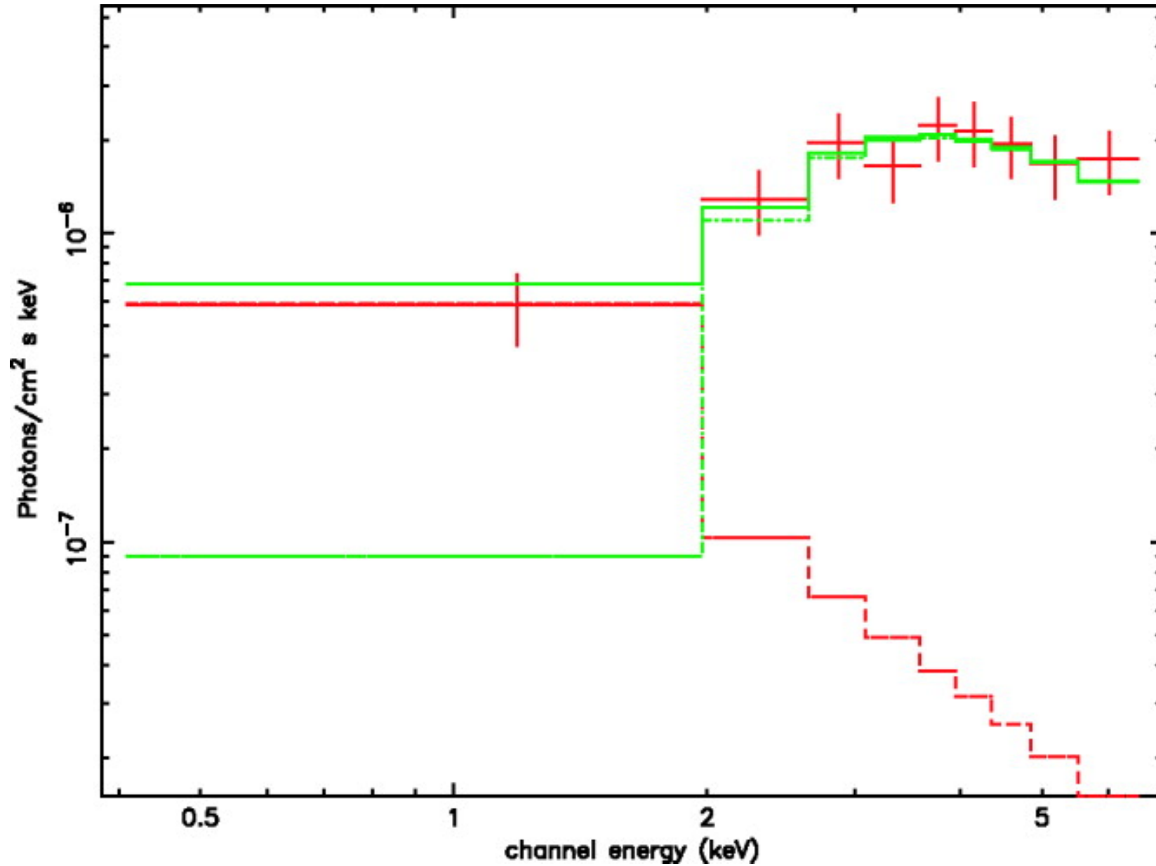
Fig. 7. from Shock Heating in the Nearby Radio Galaxy NGC 3801 Croston, Kraft, & Hardcastle 2007 ApJ 660 191 doi:10.1086/513500 https://dx.doi.org/10.1086/513500
