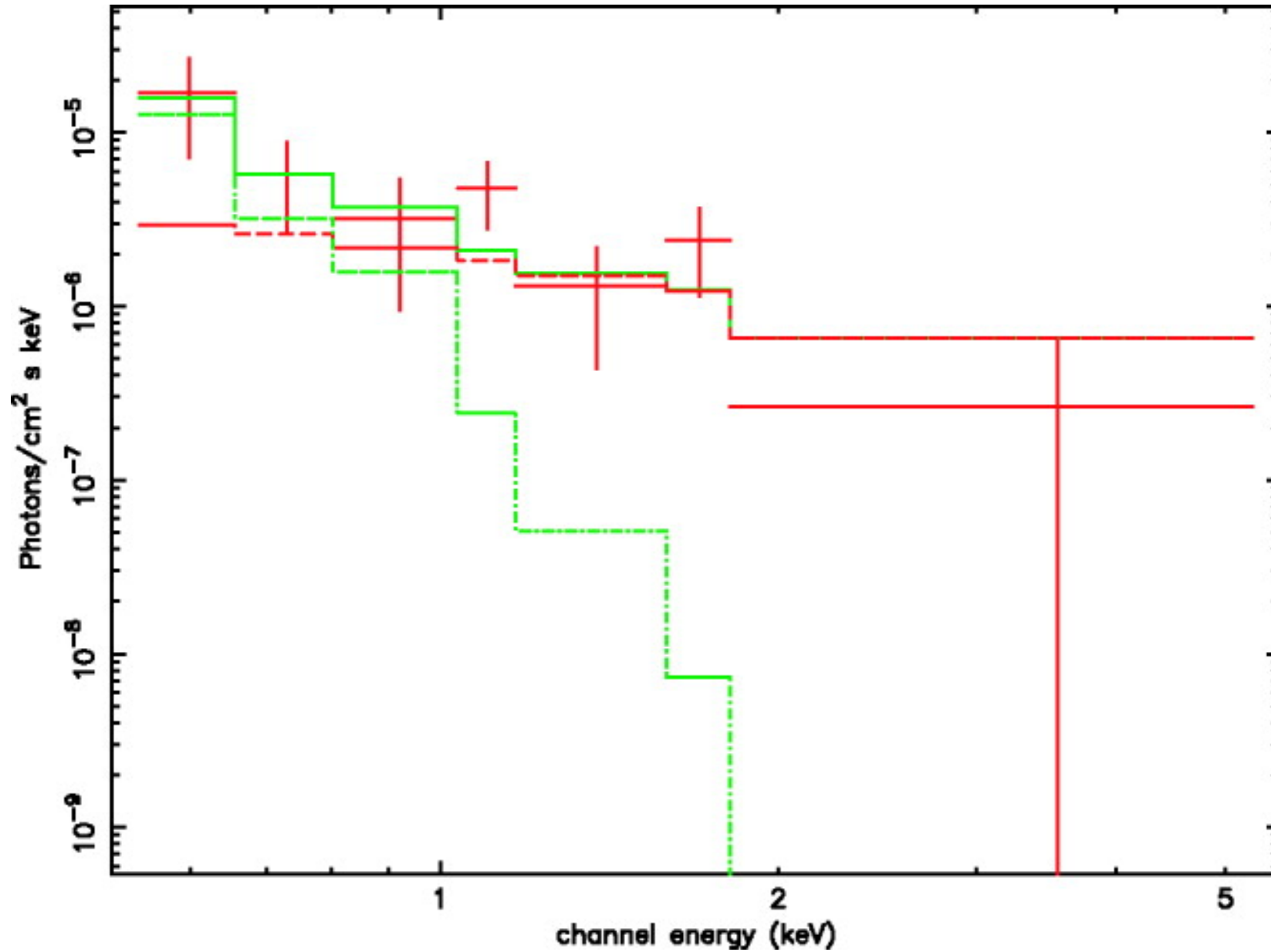
Fig. 6. from Shock Heating in the Nearby Radio Galaxy NGC 3801 Croston, Kraft, & Hardcastle 2007 ApJ 660 191 doi:10.1086/513500 https://dx.doi.org/10.1086/513500
