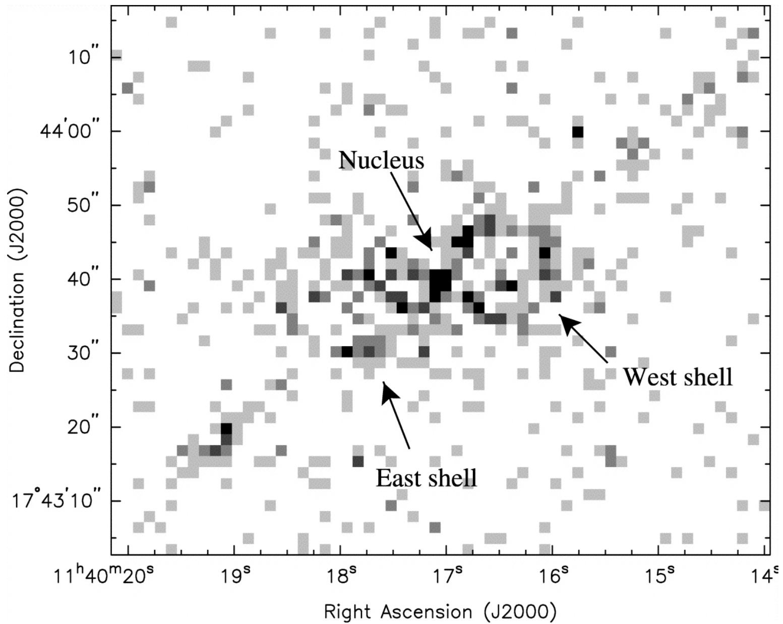
Fig. 1. from Shock Heating in the Nearby Radio Galaxy NGC 3801 Croston, Kraft, & Hardcastle 2007 ApJ 660 191 doi:10.1086/513500 https://dx.doi.org/10.1086/513500
