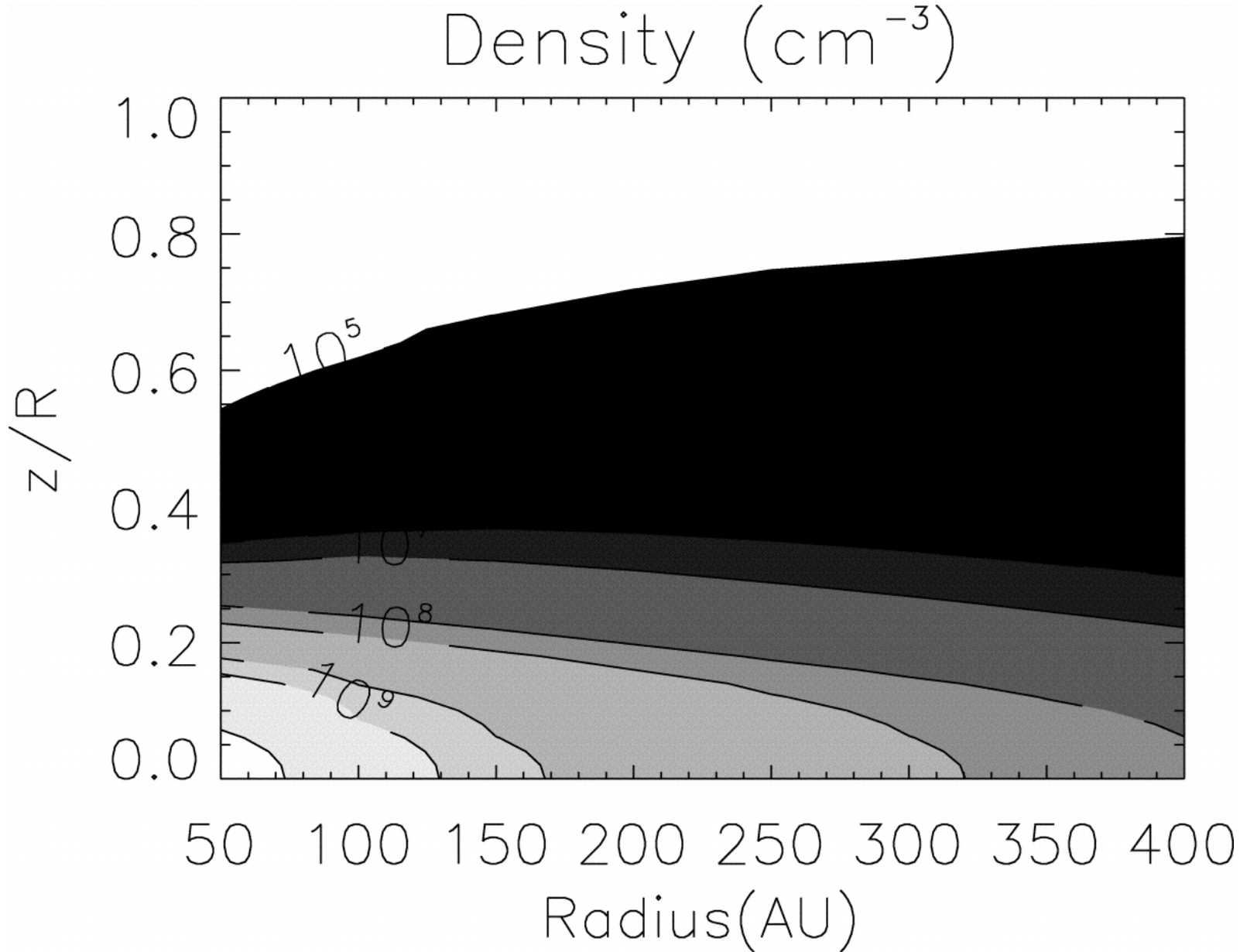
Fig. 1. from The Chemistry of Multiply Deuterated Molecules in Protoplanetary Disks. I. The Outer Disk Willacy 2007 ApJ 660 441 doi:10.1086/512796 https://dx.doi.org/10.1086/512796 © 2007. The American Astronomical Society. All rights reserved. Printed in U.S.A.
