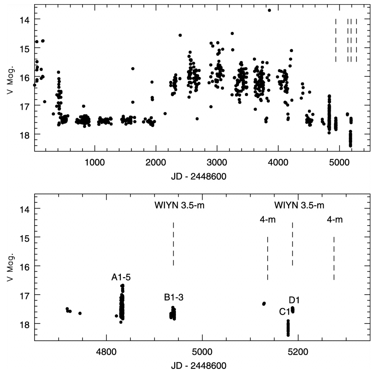
Fig. 1. from A Photometric and Spectroscopic Study of the Cataclysmic Variable ST LMi during 2005–2006 Kafka et al. 2007 AJ 133 1645 doi:10.1086/511785 https://dx.doi.org/10.1086/511785 © 2007. The American Astronomical Society. All rights reserved. Printed in U.S.A.
