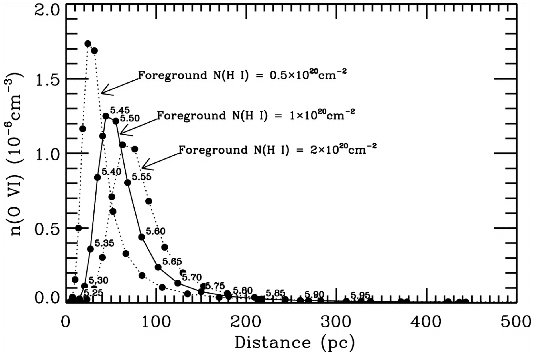
Fig. 5. from The Galactic Halo's O VI Resonance Line Intensity Shelton, Sallmen, & Jenkins 2007 ApJ 659 365 doi:10.1086/511152 https://dx.doi.org/10.1086/511152
