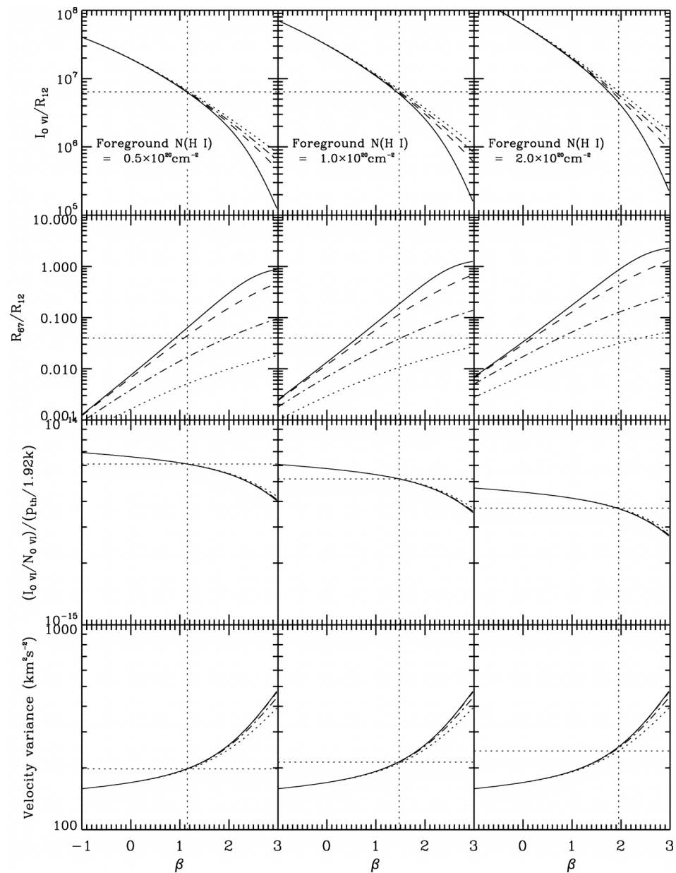
Fig. 4. from The Galactic Halo's O VI Resonance Line Intensity Shelton, Sallmen, & Jenkins 2007 ApJ 659 365 doi:10.1086/511152 https://dx.doi.org/10.1086/511152
