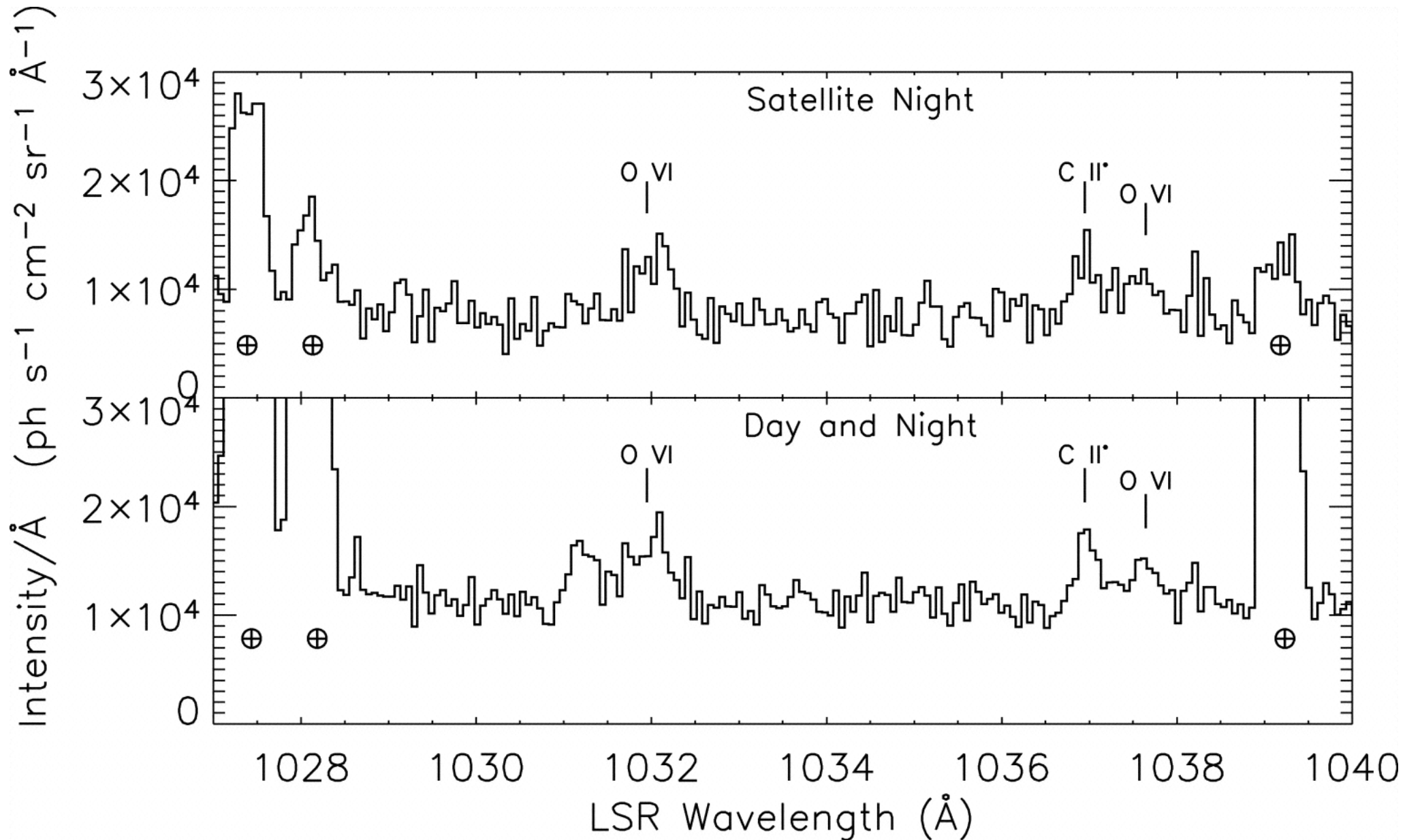
Fig. 2. from The Galactic Halo's O VI Resonance Line Intensity Shelton, Sallmen, & Jenkins 2007 ApJ 659 365 doi:10.1086/511152 https://dx.doi.org/10.1086/511152
