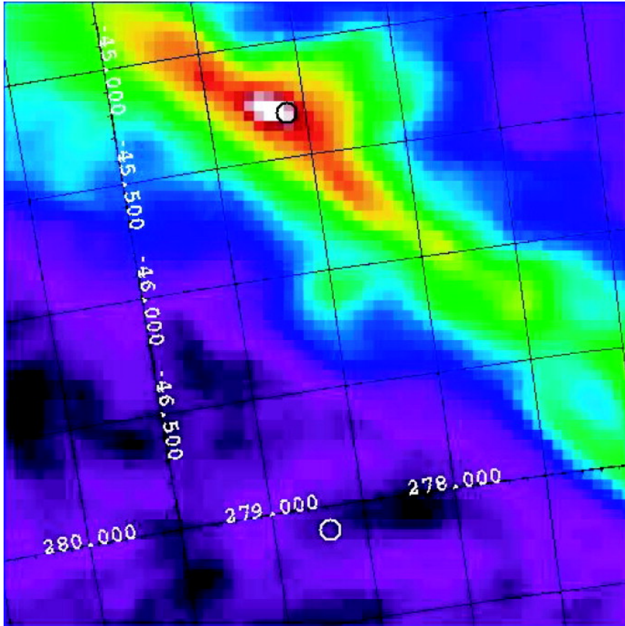
Fig. 1. from The Galactic Halo's O VI Resonance Line Intensity Shelton, Sallmen, & Jenkins 2007 ApJ 659 365 doi:10.1086/511152 https://dx.doi.org/10.1086/511152
