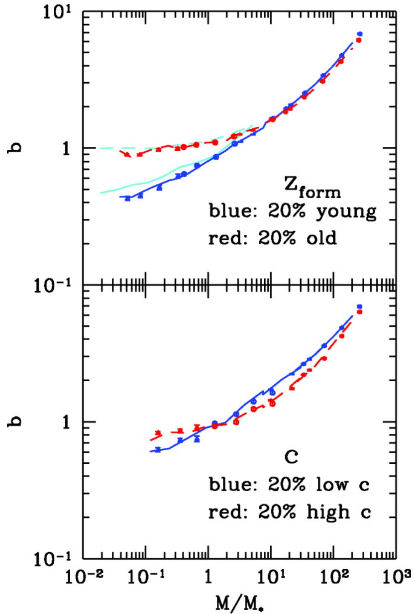
Fig. 2. from The Dependence of Dark Halo Clustering on Formation Epoch and Concentration Parameter Jing, Suto, & Mo 2007 ApJ 657 664 doi:10.1086/511130 https://dx.doi.org/10.1086/511130
