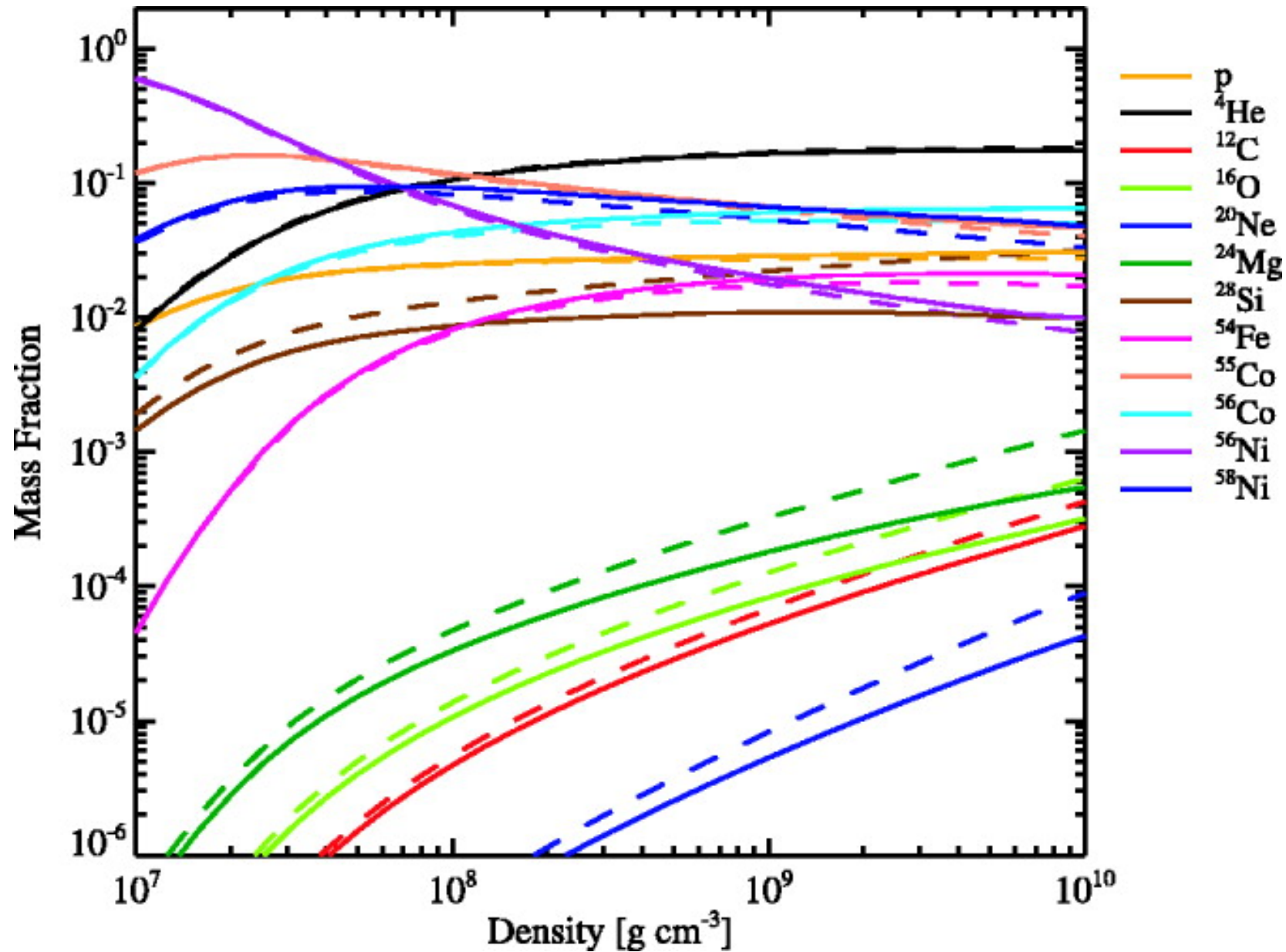
Fig. 9. from Capturing the Fire: Flame Energetics and Neutronization for Type Ia Supernova Simulations Calder et al. 2007 ApJ 656 313 doi:10.1086/510709 https://dx.doi.org/10.1086/510709 © 2007. The American Astronomical Society. All rights reserved. Printed in U.S.A.
